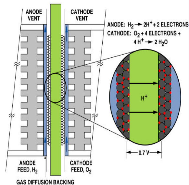
CROSS SECTION OF POLYMER ELECTROLYTE FUEL CELL
